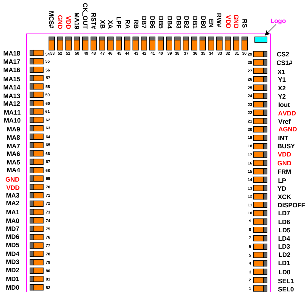
Figure 10-1 : Bonding Pad
