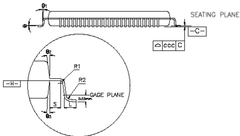
Figure 10-6 : LQFP-100Pin(12x12 mm) Mechanical(2)
