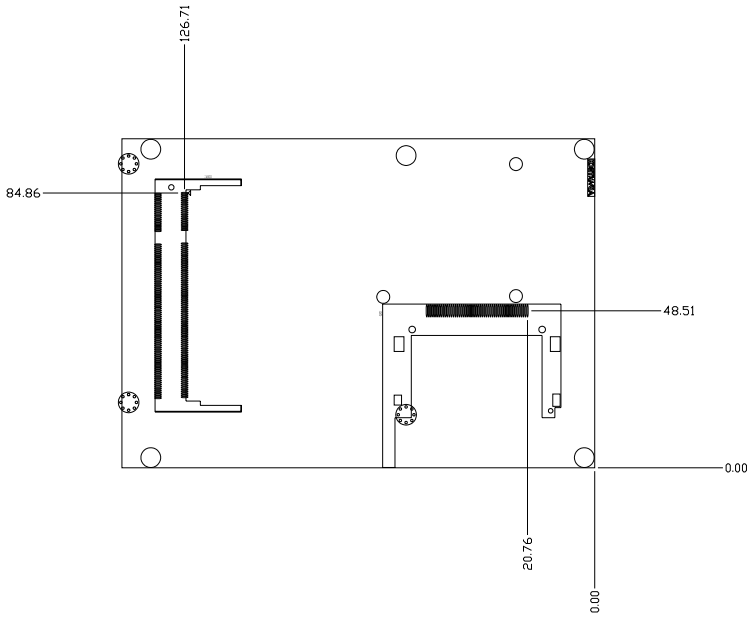
Figure F.2: PCM-9387 Mech Drawing (Solder Side)
