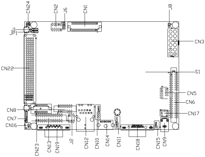
Figure 2.1: Jumpers and Connectors Drawing (component side)
