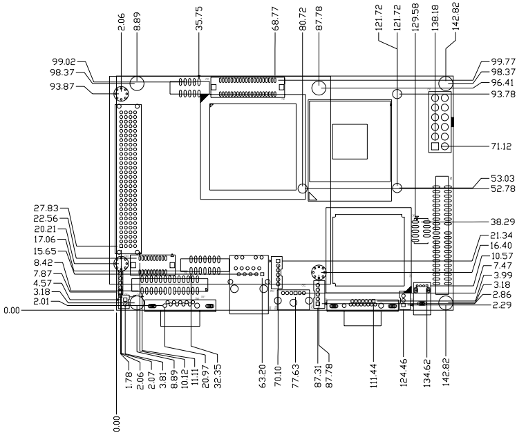
Figure F.1: PCM-9387 Mech Drawing (Component)
