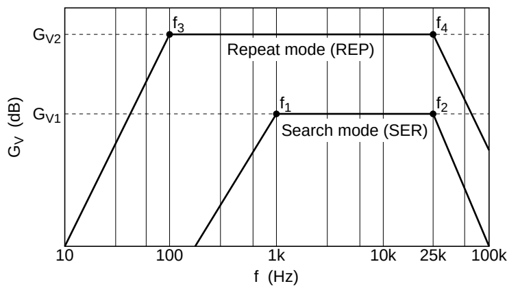
Figure 5 Frequency Response
