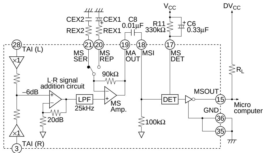
Figure 4 Music Sensor Block Diagram
