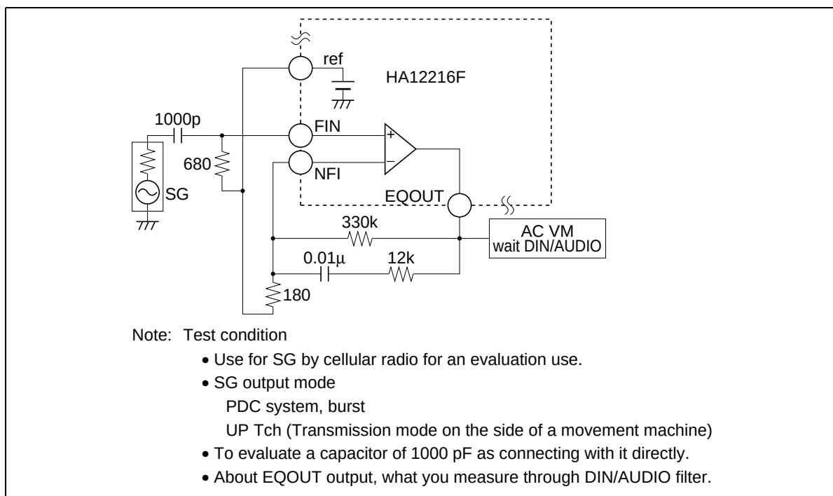
Figure 7 Test Circuit
