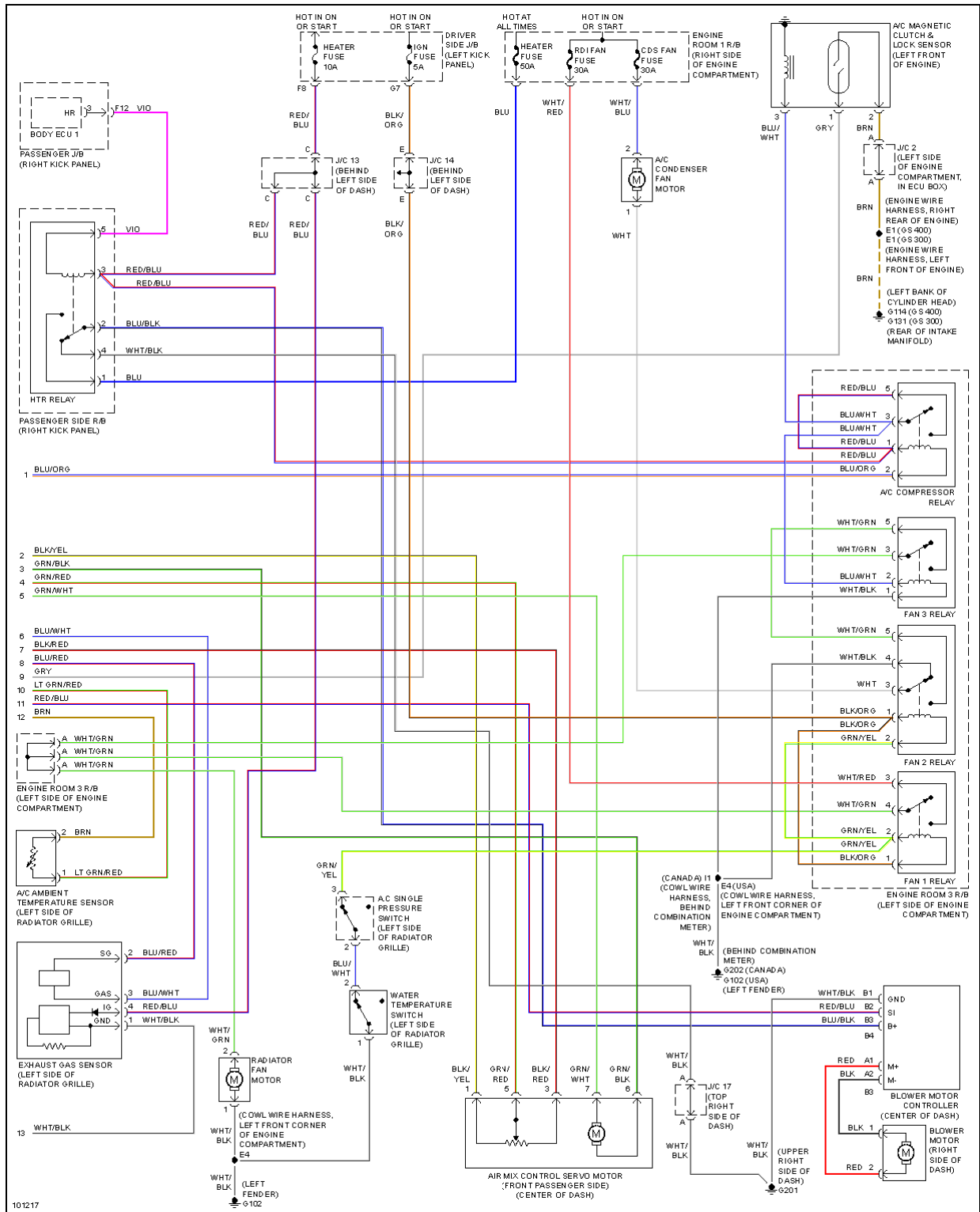
Fig. 2: Air Conditioning Circuits (2 of 2)
