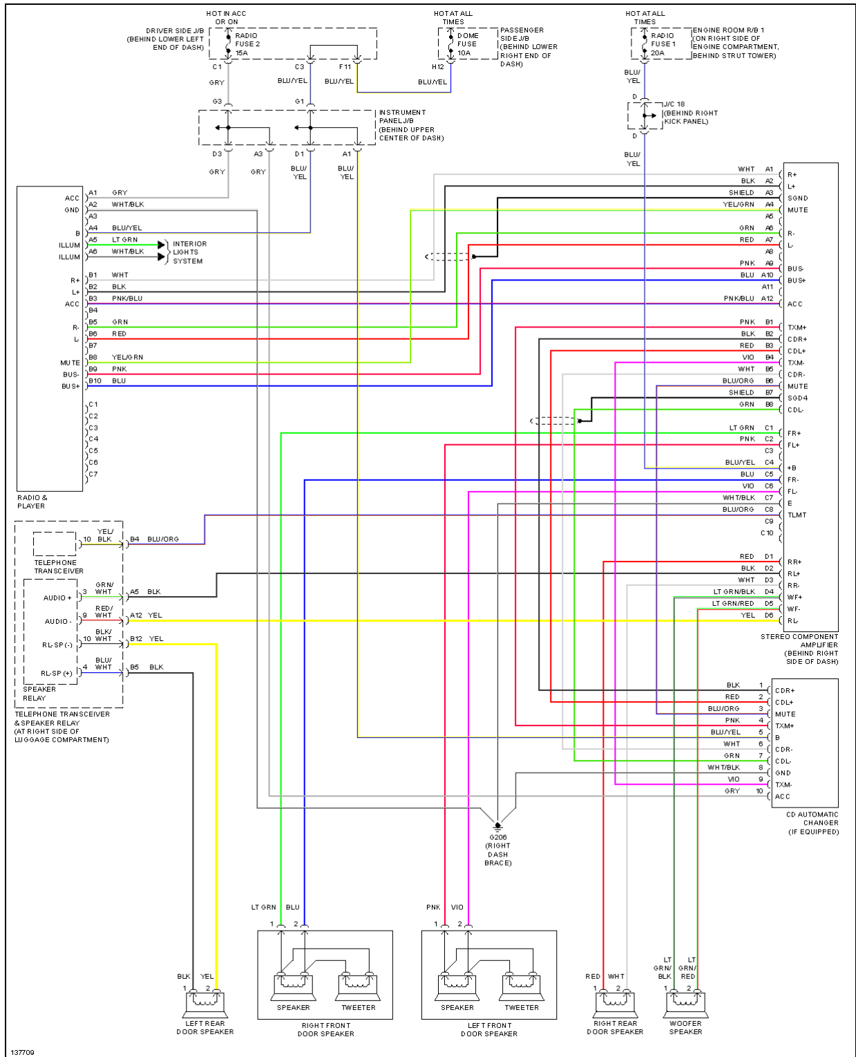
Fig. 56: Radio Circuits, Except Nakamichi W/O Navigation
